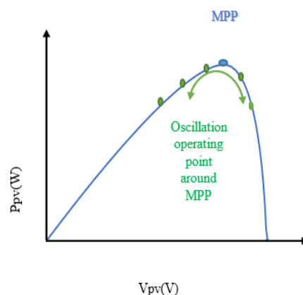
Fig. 6. Oscillation operating point during P&O operation.
