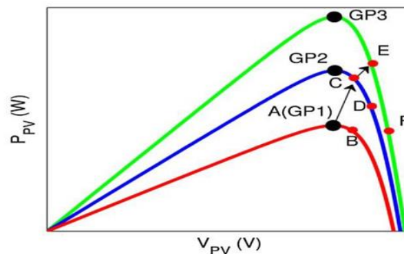
Fig. 12. P-V curve of PV module under changing irradiance [21].
