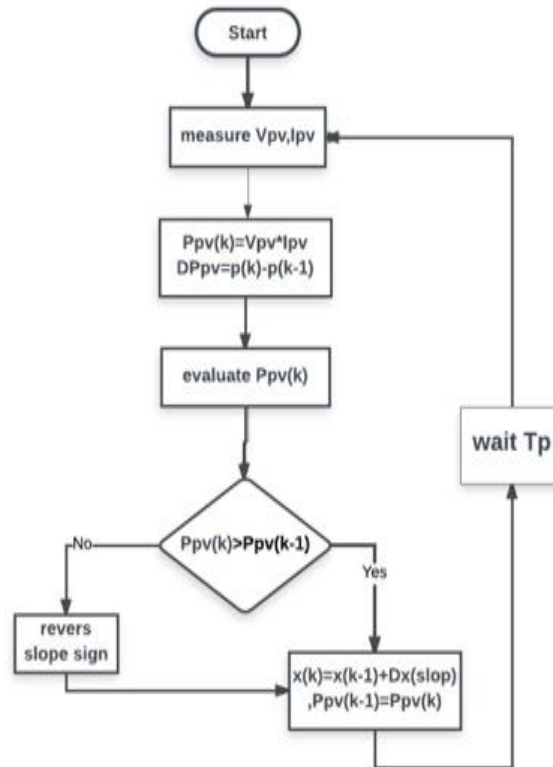
Fig. 5. Flowchart of P&O techniques.
