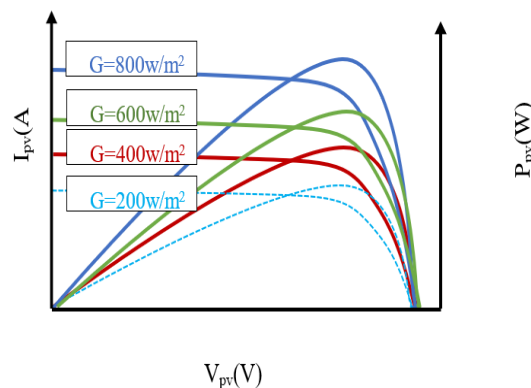
Fig. 2. I-V and P-V curves under various irradiance.
