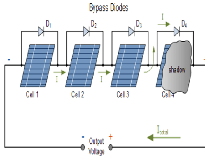
Fig. 13. one cell under partial shading.
