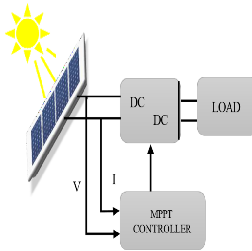
Fig. 3. Structure of photovoltaic system with MPPT controller.
