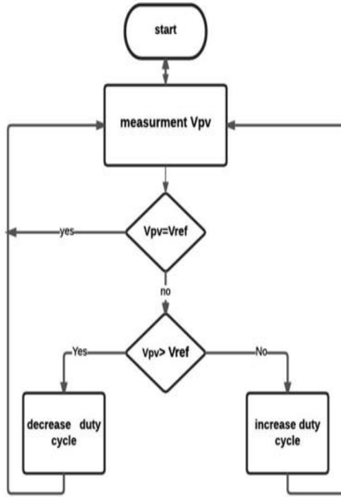
Fig. 4. Flowchart of FOCVT algorithm.
