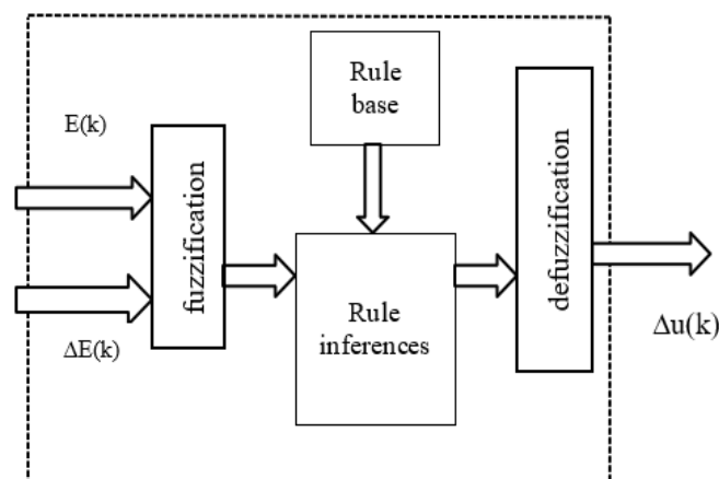
Fig. 9. The basic structure of fuzzy logic control.
