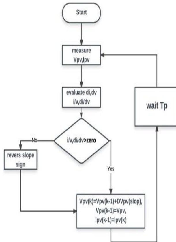
Fig. 8. flowchart of Incremental conductance method.
